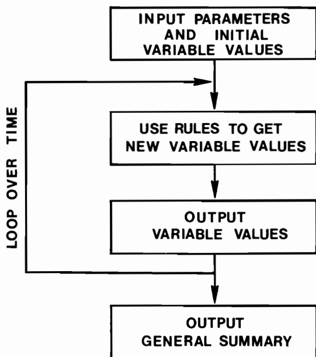
FIGURE A.11 Most dynamic simulation models have the same basic format: rules for change that can be applied repeatedly.
