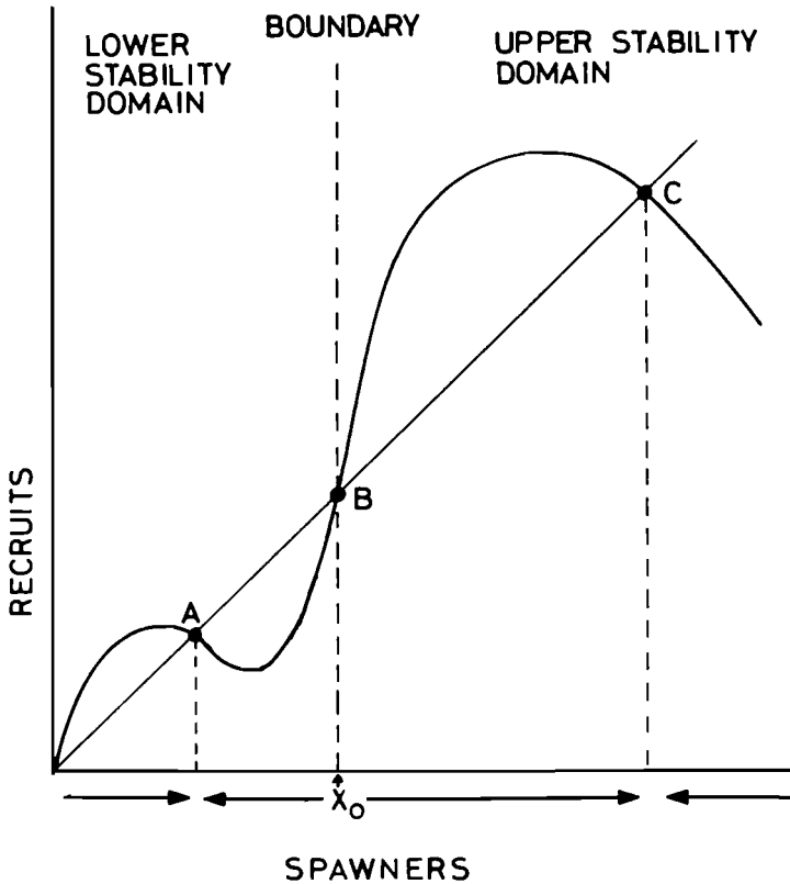
FIGURE 12.11 A recruitment curve showing the effect of predation mortality. The diagonal line is the replacement line, where recruits equal spawners. After Peterman (1977b).
