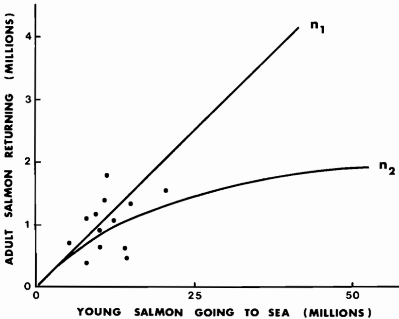
FIGURE 12.16 Historical abundances of juvenile salmon of this hypothetical stock have not produced data that permit us to distinguish between alternative models of ocean limitation ( n_1 : no limitation; n_2 : a saturation level exists).
