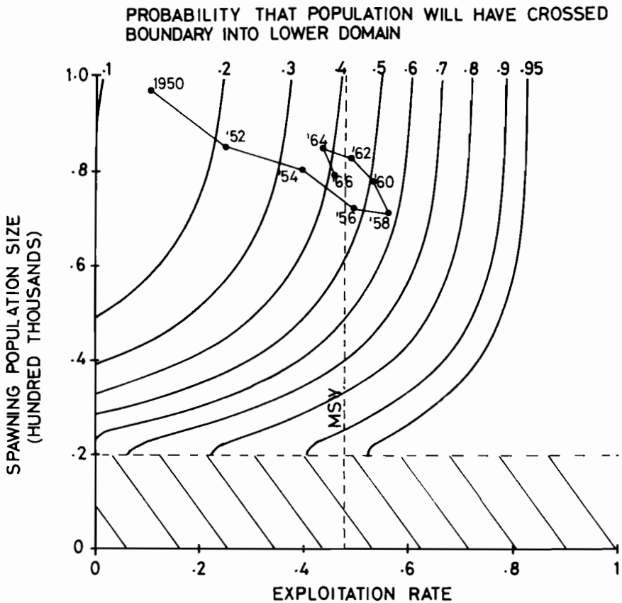
FIGURE 12.13 The contours give the probability that a stock will cross into the lower domain if a given exploitation rate is applied to its offspring. Superimposed on these contours is the time course of a hypothetical developing fishery. The maximum sustainable yield exploitation rate (MSY) is indicated by the vertical dotted line. Below the dashed line, there exists only a single domain of attraction — in this case, the lower domain. After Peterman (1977b).
