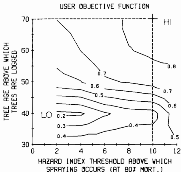
FIGURE A.17 The hypothetical objective function surface derived by giving a relative importance weighting of 0.3 to minimization of years spraying done and 0.7 to maximization of profits (see text). The general form of the objective function is U = \sum_i W_i I_i , where W_i is the relative importance weighting of the i -th indicator ( \sum_i W_i = 1.0 ) and I_i is the value of the i -th indicator scaled from 0 to 1 (1.0 is the lowest value of I_i if that indicator is being minimized or the highest value if it is being maximized). The "best" management option, given the specified objective, is to cut trees above age 70 and to spray the site when the hazard index gets above 10.
