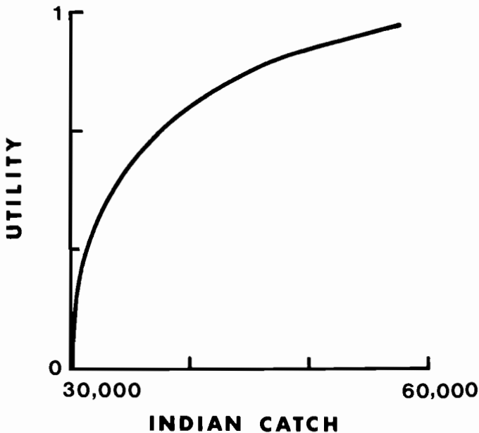
FIGURE 12.3 A sample utility function for an Indian catch indicator.
