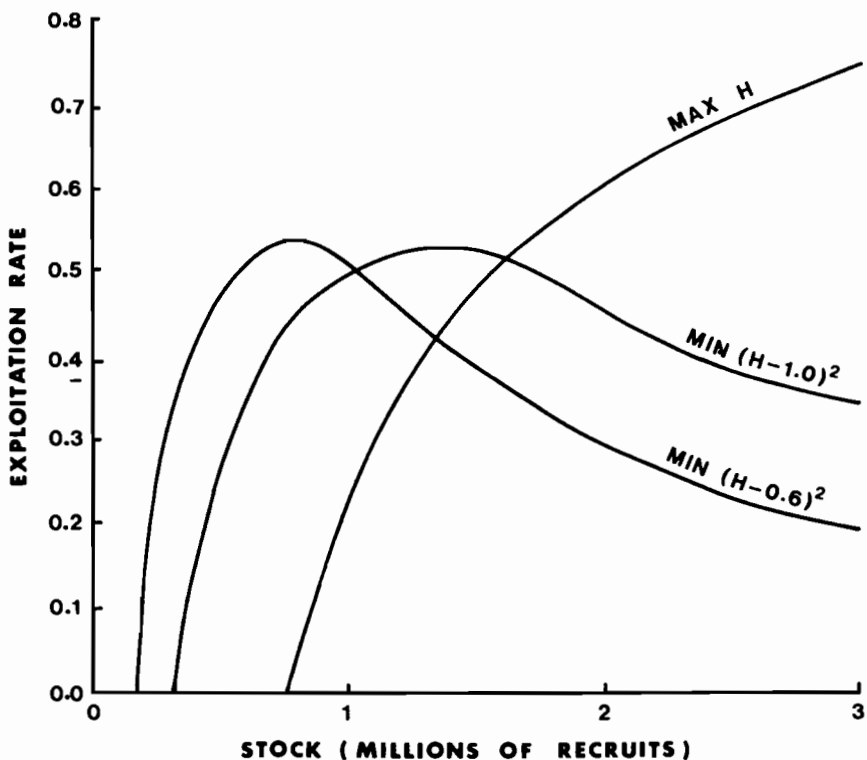
FIGURE 12.5 Optimal harvest strategies that would achieve one of three different management objectives: maximum sustainable yield (Max H ); minimization of the variance in catches around a mean value of 1.0 million fish [ \text{Min } (H - 1.0)^2 ]; and minimization of the variance in catches around a mean value of 0.6 million fish [ \text{Min } (H - 0.6)^2 ]. Redrawn from Walters (1975b).
