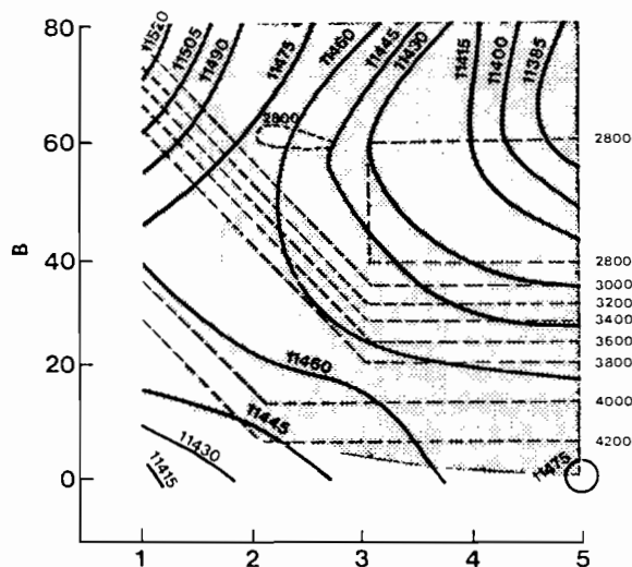
FIGURE 14.13 Optimum solution (circle) for maximizing total net benefits under a 50-year time horizon, constrained by an average hydroelectric production of 3,750 GWh and an ecological deterioration equal to or less than 10% (shaded area covers the non-possible solutions).
