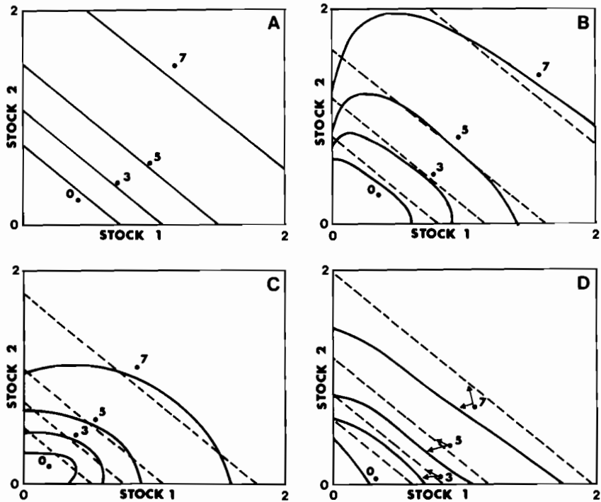
FIGURE 12.7 Isoclines of optimal harvest rates for a fishery that simultaneously harvests two stocks. Derivations from dynamic programming are represented by solid lines, from fixed escapements by dashed lines. Four different cases of production parameter combinations are shown. In Case A , both stocks have the same production parameters and the solutions from dynamic programming and fixed escapement are identical. In Cases B , C , and D the two stocks differ in their production parameters. After Hilborn (1976).
