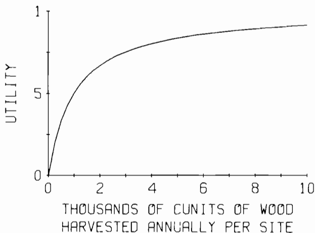
FIGURE A.19 A hypothetical example of the utility, or "satisfaction gained" by having different amounts of wood harvested in New Brunswick each year.
