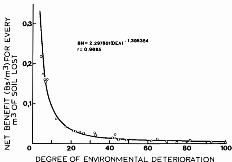
FIGURE 14.12 Net benefits obtained for every m 3 of lost soil (Bs/m 3 ) as a function of the degree of ecological deterioration of the basin.
