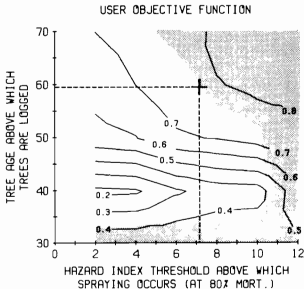
FIGURE A.18 When a constraint is applied to the objective of Fig. A.17, by requiring more than 6000 cunits to be harvested annually, a non-feasible set of management options (in the shaded area) are delineated. This constraint region shifts the "best" management option to cutting age of 59 years and hazard index threshold of a little over 7. This particular constraint region is derived from the location of the 6000 cunit contour on the "average annual cunits harvested" nomogram shown in Fig. A.15.
