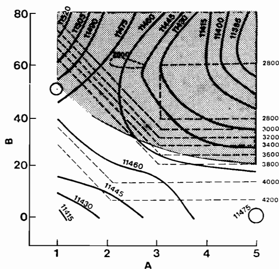
FIGURE 14.15 Optimum solutions (circles) for maximizing total net benefits under a 50-year time horizon, constrained by an average hydroelectric production of 3,750 GWh and an ecological deterioration equal to or less than 30% (shaded area covers the non-possible solutions).
