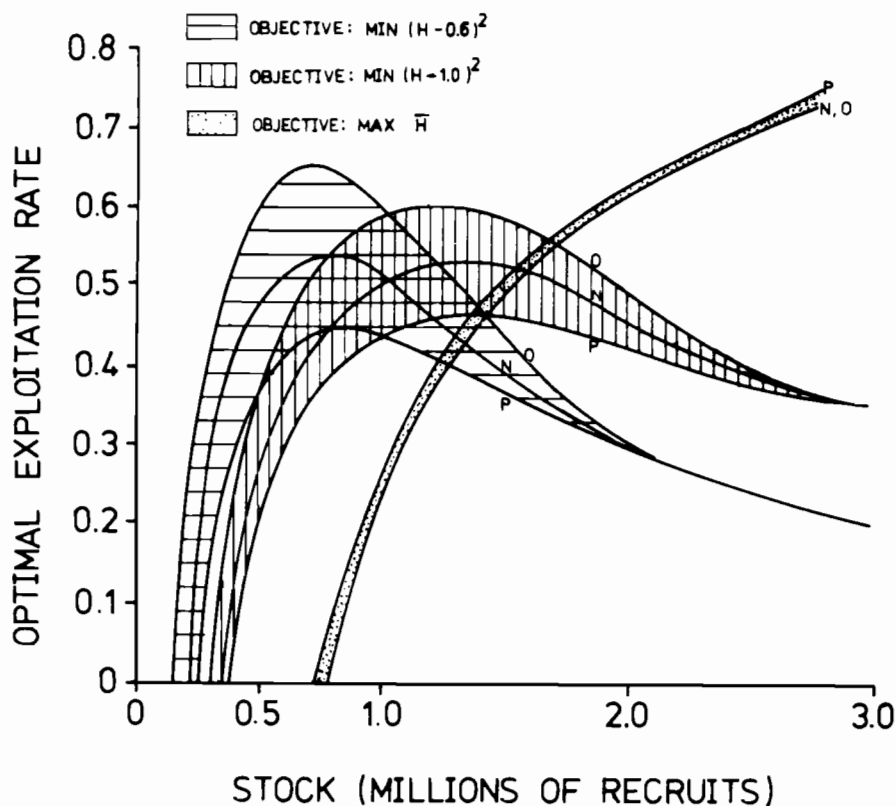
FIGURE 12.6 Optimal harvest strategies for three different objective functions using the optimistic (O), natural (N), and pessimistic (P) probability distributions for the production parameter data. After Walters (1975b).
