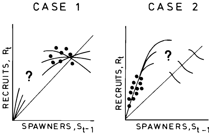
FIGURE 12.9 Management situations that permit simplified adaptive optimization. Case 1: newly developing fishery, \beta known and \alpha uncertain. Case 2: older fishery with stock depleted below unfished level, \alpha known and \beta uncertain. After Walters and Hilborn (1976).
