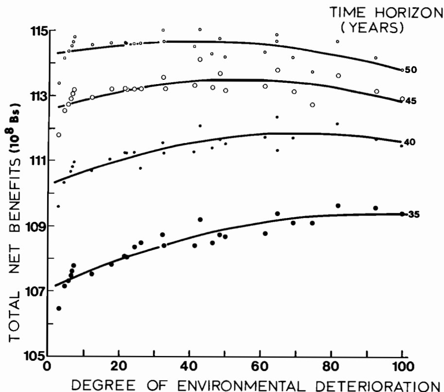
FIGURE 14.11 Total net benefit as a function of the degree of ecological deterioration of the basin, evaluated at 4 time horizons (35, 40, 45, and 50 years).
