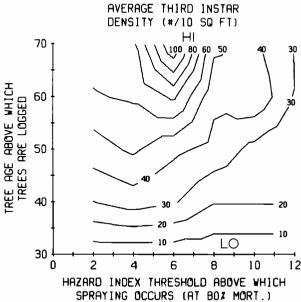
FIGURE A.14 Contour lines can be drawn through the “heights” of the indicator shown in Fig. A.13 to yield a “nomogram,” or response surface.
