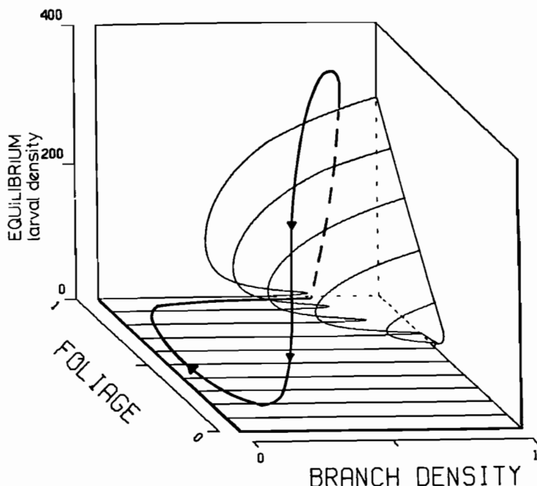
FIGURE 11.10 Budworm manifold (position of all equilibrium levels of budworm) for different amounts of living foliage per branch and different densities of branches per acre. The trajectory shows a typical path through this space, describing one outbreak cycle in an unmanaged world.
