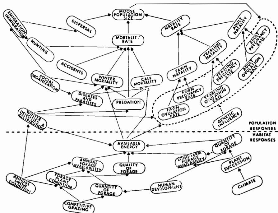
FIGURE 15.1 Simplified network of population and habitat features that combine to control a population's density (in this case, a moose population).
