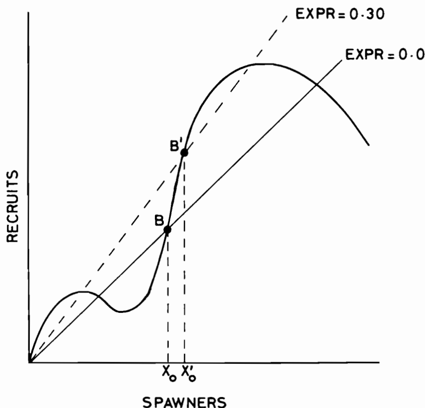
FIGURE 12.12 The slope of the replacement line changes when the exploitation rate (EXPR) is altered. The boundary population size then changes from X_0 to X'_0 . After Peterman (1977b).
