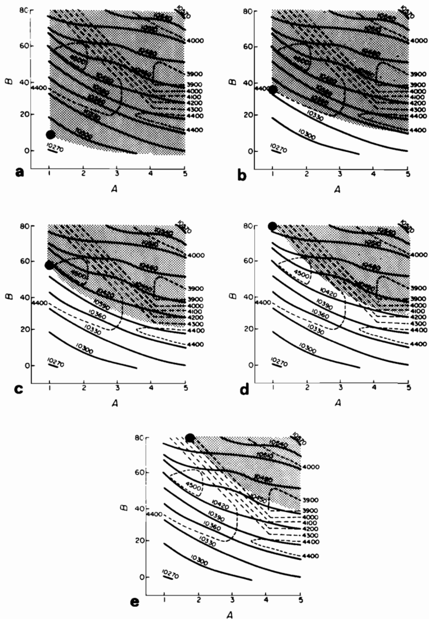
FIGURE 14.18 Sequence of optimum decisions similar to Figures 13–17 but for a 30-year time horizon.
