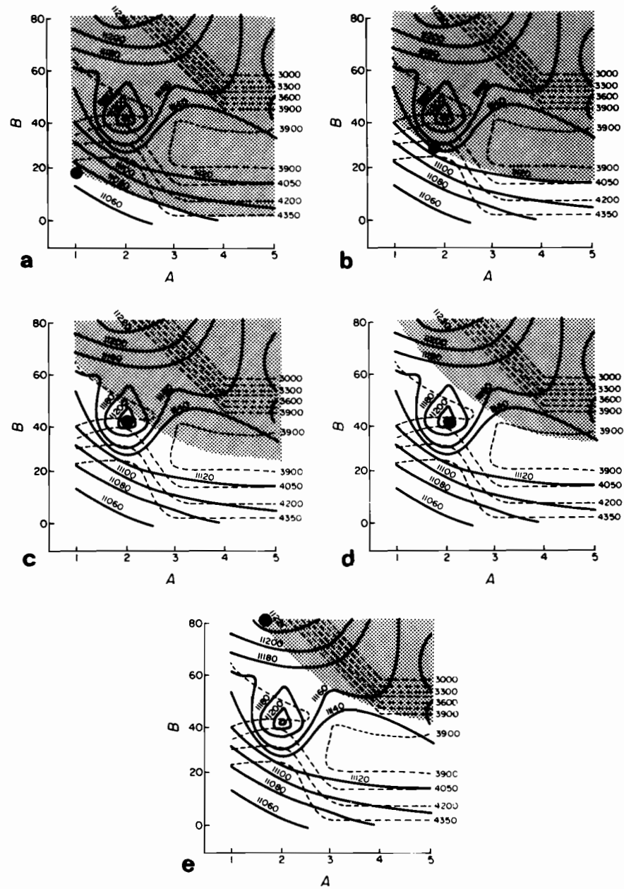
FIGURE 14.19 Sequence of optimum decisions similar to Figures 13–17, but for a 40-year time horizon.
