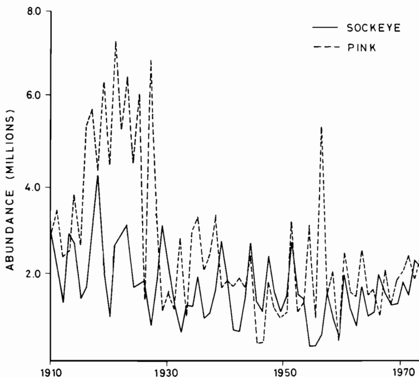
FIGURE 12.1 Historical changes in Skeena River (British Columbia) salmon abundance.
