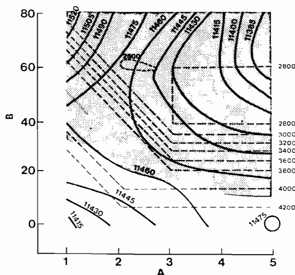
FIGURE 14.14 Optimum solution (circle) for maximizing total net benefits under a 50-year time horizon, constrained by an average hydroelectric production of 3,750 GWh and an ecological deterioration equal to or less than 20% (shaded area covers the non-possible solutions).
