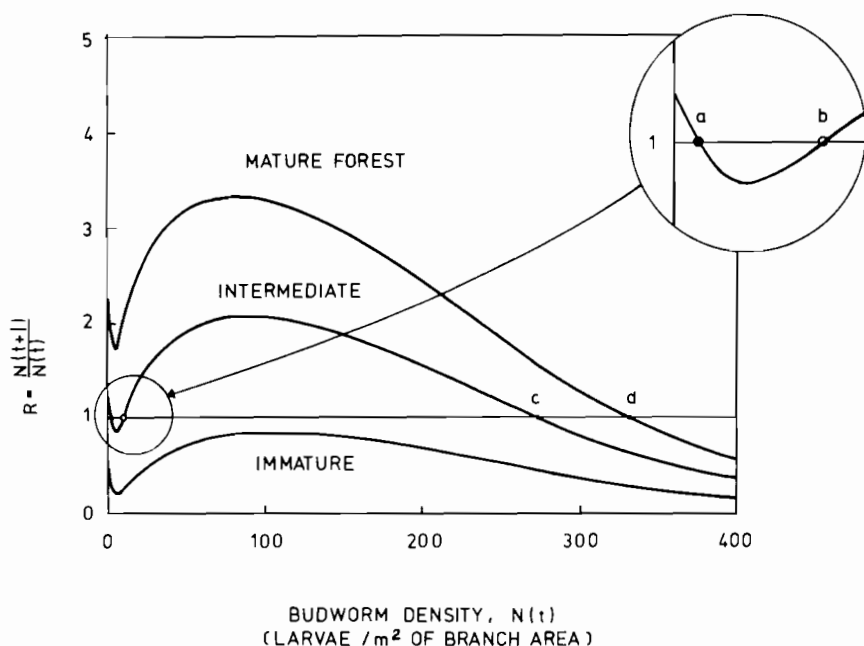
FIGURE 11.9 Growth-rate curves for budworm populations at various budworm densities and three forest conditions. Potential equilibria occur whenever the growth rate intersects the horizontal “replacement” line.
