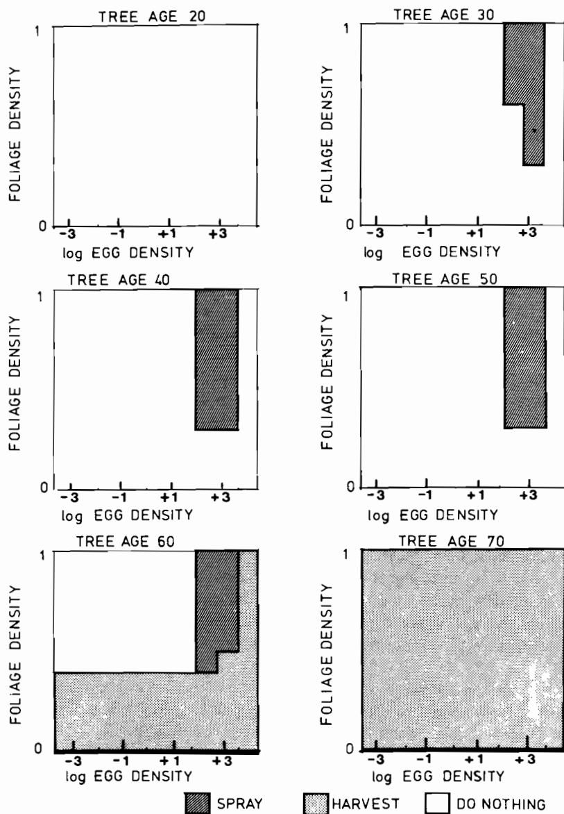
FIGURE 11.12 Representative policy tables generated by the Winkler-Dantzig optimization. A separate table is provided for each age of tree (or, in practice, age of stand). The table tells what management act should optimally be applied to the tree as a function of the tree's present complement of foliage (foliage density) and its resident budworm egg density (here plotted as the logarithm of egg density). Available management options are to do nothing, to spray, and to harvest or log the tree.
