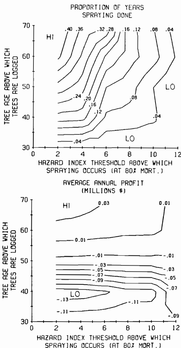
FIGURE A.16 Two component indicators of a simple, hypothetical objective. The profits indicator only shows the total dollars profit to the forest industry where the sale price is $45 per cunit and the costs of logging are as shown by that indicator in Fig. A.15. Note that if "proportion of years spraying done" should be minimized and profits maximized, there will have to be some compromise, as the optimal regions for these two indicators are at different corners of the graphs.
