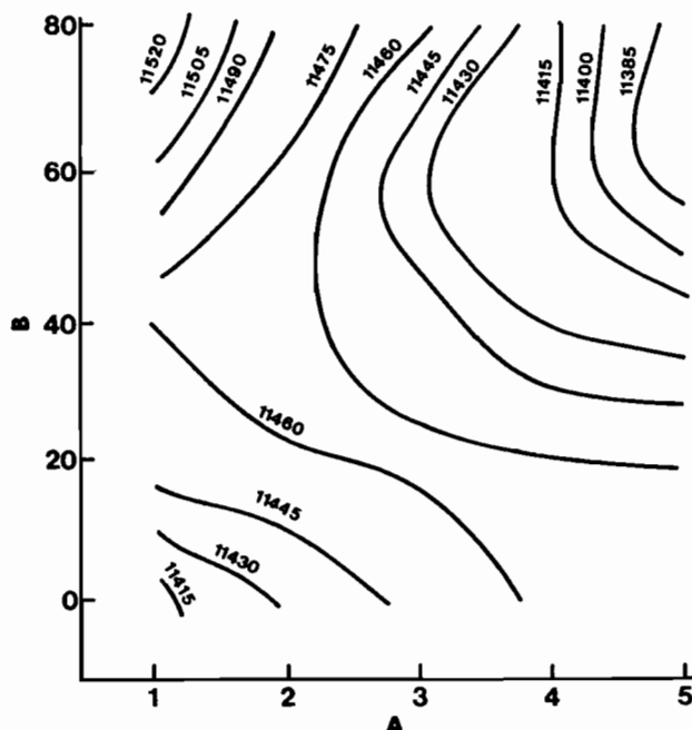
FIGURE 14.10 Total net benefits (millions of Bs) in year 50 of simulation corresponding to the 25 intervention strategies.
