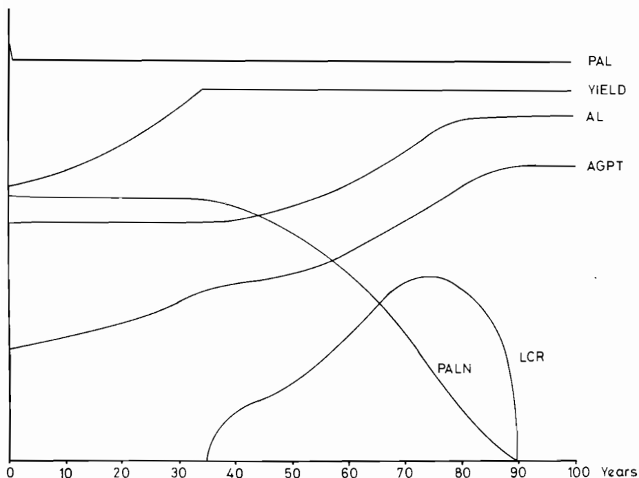
FIGURE A.6 Output of the full simulation model. The names of the variables are the same as in Figure A.4. Their ranges during the simulation are: AL ( 0.634\text{E}6 - 0.109\text{E}7 ); PALN ( 0 - 0.459\text{E}6 ); YIELD ( 0.65\text{E}1 - 0.10\text{E}2 ); PAL ( 0.10929\text{E}7 - 0.10930\text{E}7 ); AGPT ( 0.195\text{E}16 - 0.517\text{E}16 ); \Delta\text{LC} ( 0 - 131\text{E}5 ).
