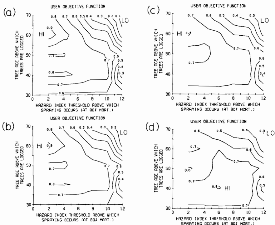
FIGURE A.20 An example of how shifts in relative importances of indicators can change the “best” management options (see text). The areas marked “HI” are the high points on the objective function surfaces. (a) – relative importance weightings are 0.05 on proportion of years sprayed and 0.95 on average annual cunits logged (denoted 0.05/0.95); optimum is at (2, 60). (b) – weightings are 0.1/0.9 and optimum is also at (2, 60). (c) – weightings are 0.2/0.8 and optimum is still (2, 60). (d) – weightings are 0.3/0.7 and optimum now changes to (6, 40).
