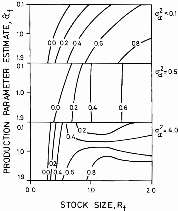
FIGURE 12.10 Isopleths of optimal exploitation rates for various stock sizes, production rate estimates ( \hat{\alpha}_t ), and uncertainties about \alpha ( \sigma_\alpha^2 ), assuming the Ricker model form is correct and equilibrium stock is known (case 1 of Figure 12.9). These results were obtained with environmental variance \sigma^2 = 0.5 and discount rate \delta = 4\% per generation. After Walters and Hilborn (1976).
