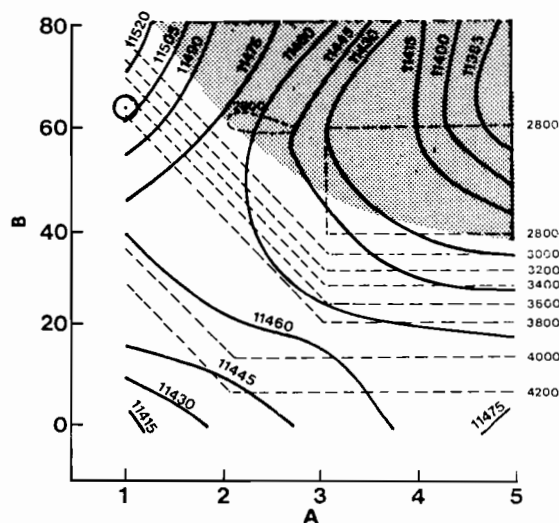
FIGURE 14.17 Optimum solution (circle) for maximizing total net benefits under a 50-year time horizon, constrained by an average hydroelectric production of 3,750 GWh and an ecological deterioration equal to or less than 50% (shaded area covers the non-possible solutions).
