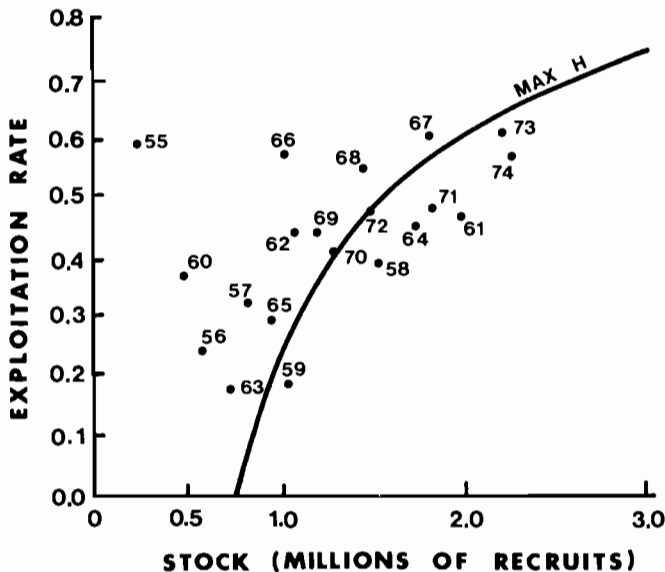
FIGURE 12.4 Harvest rate plotted against stock size. The curve is the relation that would achieve an objective of maximum sustainable yield (Max H ). Historical data for Skeena River sockeye salmon are shown for the years indicated. Redrawn from Walters (1975b).
