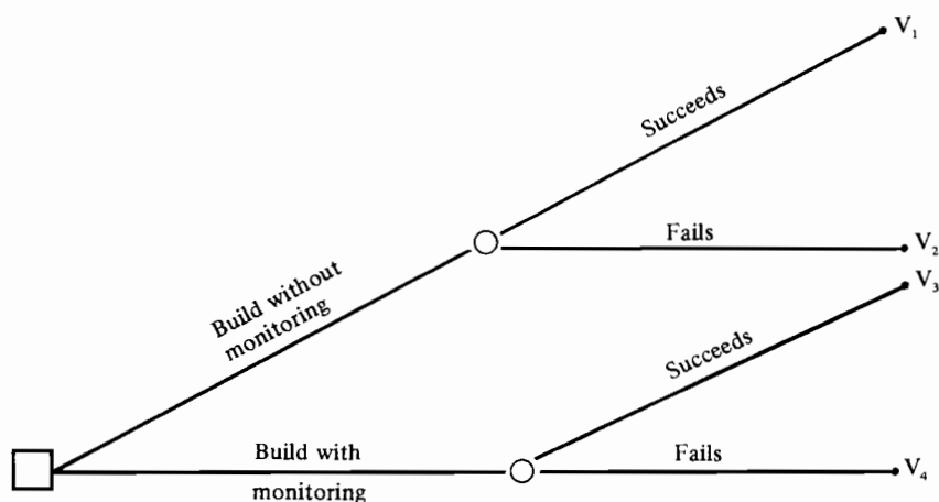
FIGURE 12.15 Decision tree for a fishery enhancement project.
