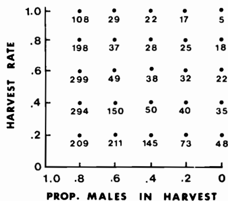
FIGURE 9.3 Second step in construction of a nomogram. See text and Table 9.1.
