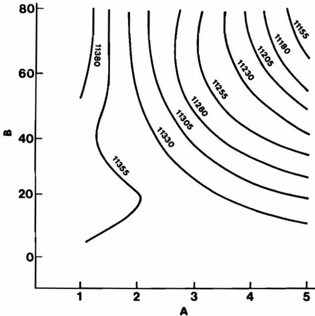
FIGURE 14.9 Net benefits produced by the hydroelectric activity (millions of Bs) in year 50 of simulation corresponding to the 25 intervention strategies.
