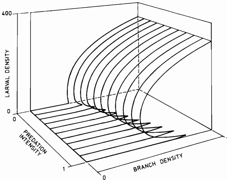
FIGURE 11.11 Budworm manifold at maximal foliage levels for different intensities of predation from 0 to the maximum occurring in nature (1) and different densities of branches per acre.
