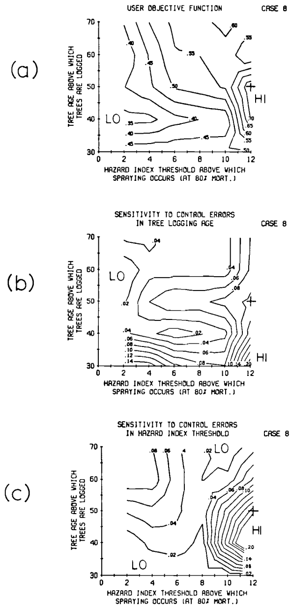
FIGURE A.21 The values of an example objective function are shown in graph (a), and the cross-hairs indicate the high point for this objective. Sensitivity to “control errors” (see text) can be analyzed by measuring the slopes of the objective function surface in both the vertical and horizontal directions, corresponding respectively to errors in tree logging age and the hazard index threshold (b) and (c).
