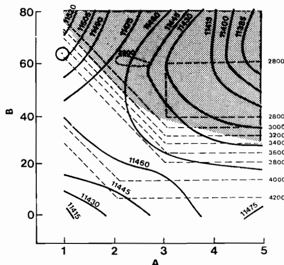
FIGURE 14.16 Optimum solution (circle) for maximizing total net benefits under a 50-year time horizon, constrained by an average hydroelectric production of 3,750 GWh and an ecological deterioration equal to or less than 40% (shaded area covers the non-possible solutions).
