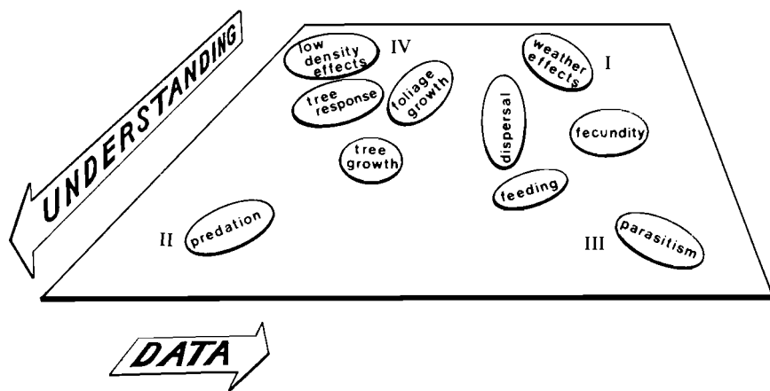
FIGURE 5.2 The location of individual ecological processes from the budworm study on the axes of amount of available data and degree of background conceptual understanding.
