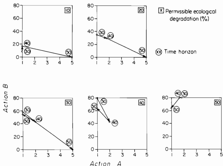
FIGURE 14.20 Three time horizon optimum decision trajectories for five different ecological deterioration constraints that maximize total net benefits with an average monthly hydroelectric production of 3,750 GWh.
