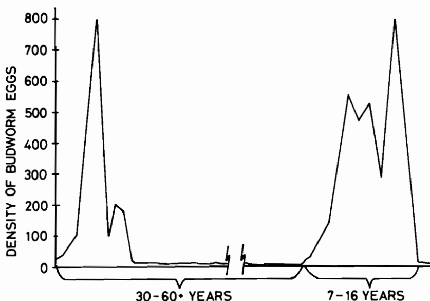
FIGURE 11.3 The pattern in time. Representative historical pattern of spruce budworm outbreak. There have been four major outbreaks since 1770. The density measure of budworm is what would occur on a typical balsam fir branch.
